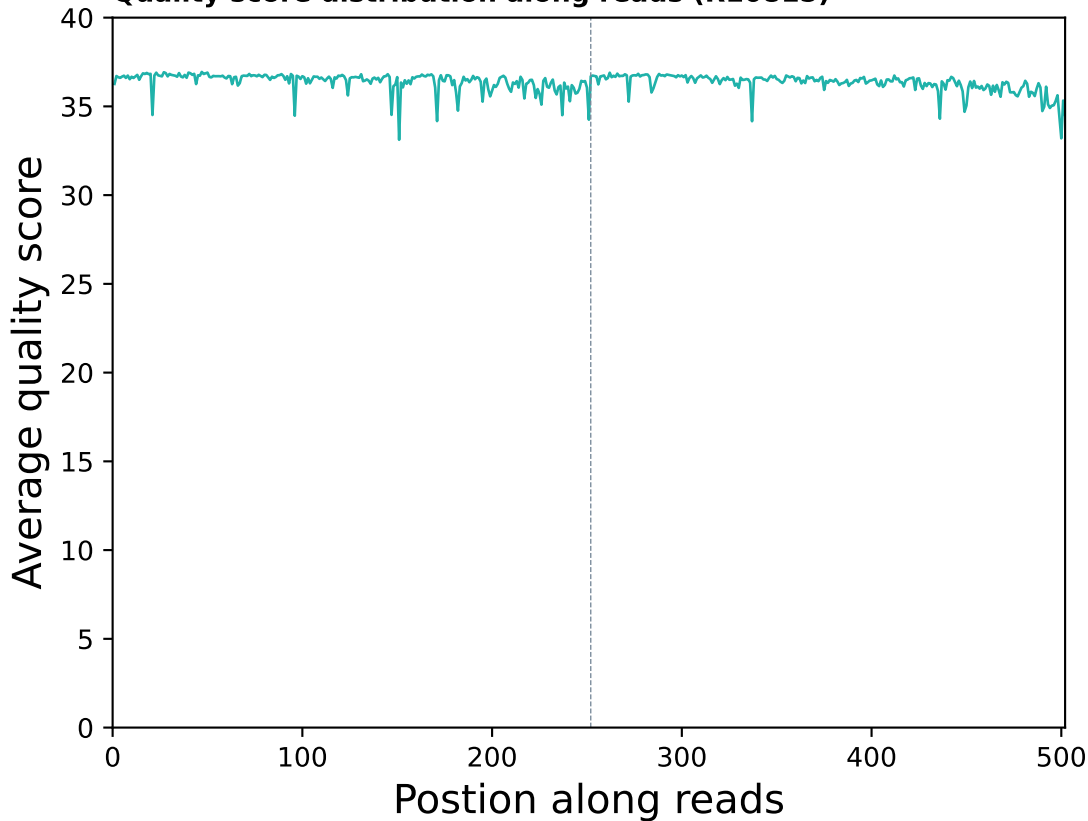
Quality score distribution along reads (R10815)
